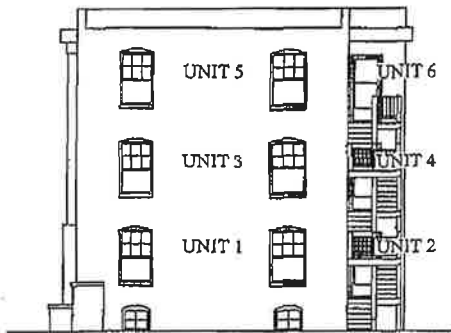
SOUTH ELEVATION BUILDING 2
