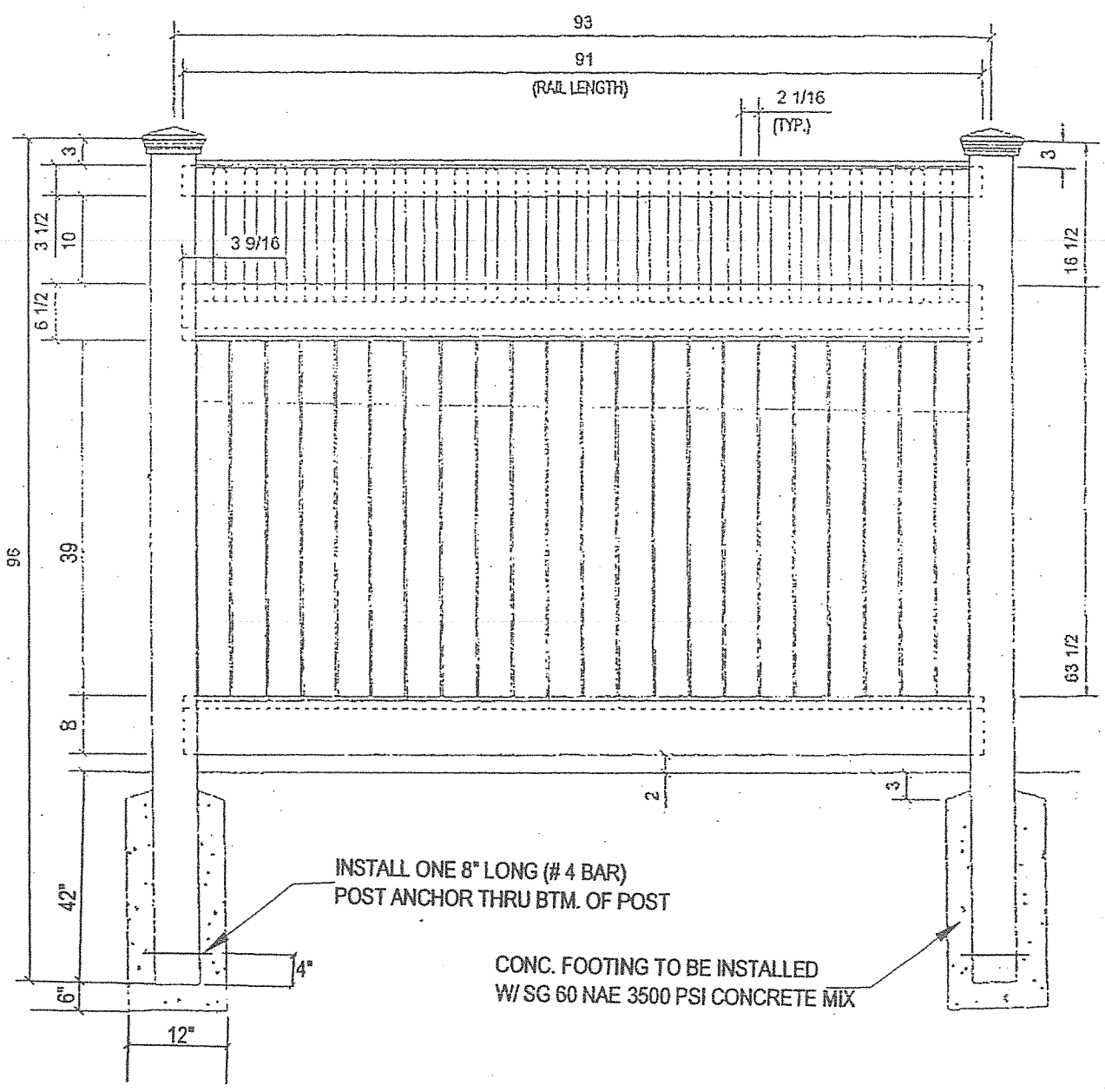
6' VINYL FENCE DETAIL
