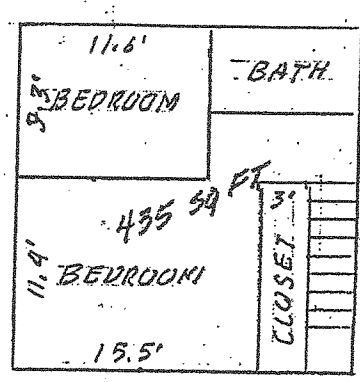
MAIN FLOOR TYPE C
