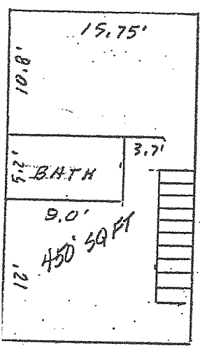
SECOND FLOOR TYPE A, B, D
